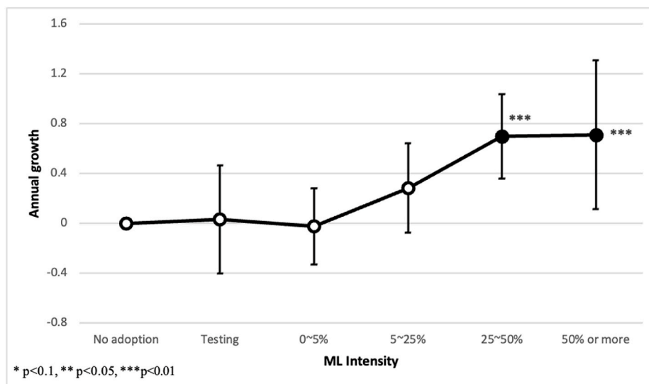
Fig. 1d. ML.
